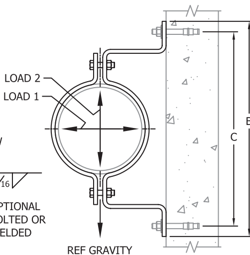
WALL MOUNTED
