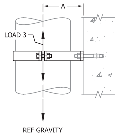
RISER APPLICATION
