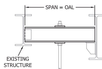
SUPPLEMENTAL STEEL
