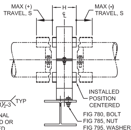
CENTERED INSTALLATION
