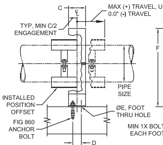
OFFSET INSTALLATION
