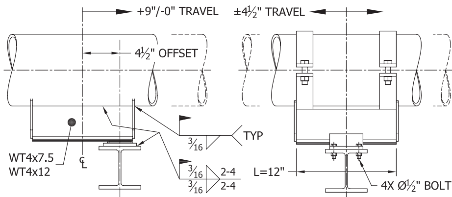
PIPE ATTACHMENT: WELDED (W) ALL TYPES
