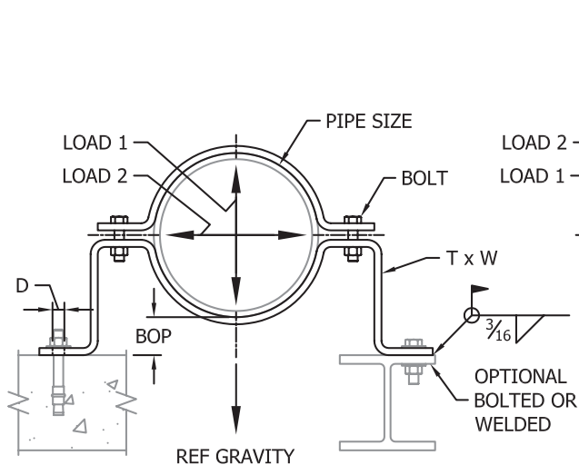
FLOOR MOUNTED
