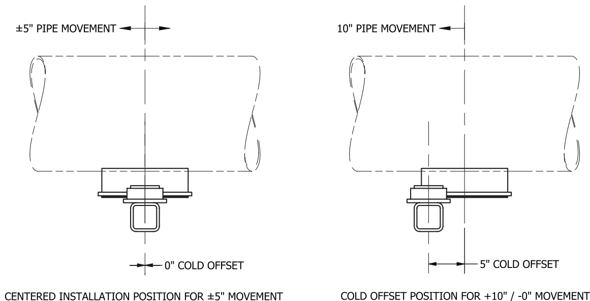
CENTERED INSTALLATION POSITION FOR \pm 5" MOVEMENT
